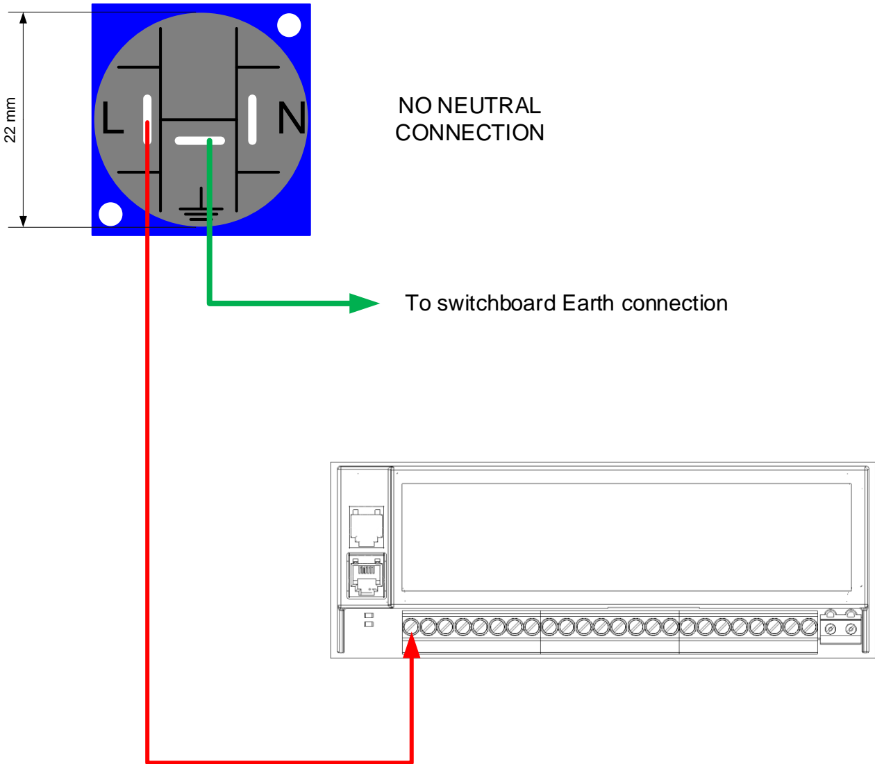
Neutrik Connector Rear View
